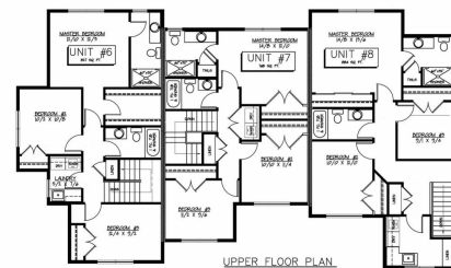
UPPER FLOOR PLAN
