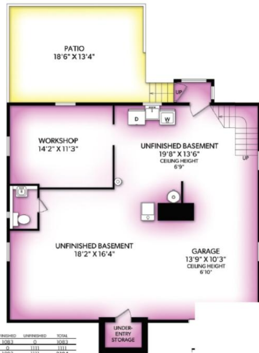
LOWER FLOOR
