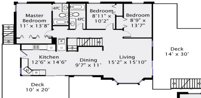
Main Level 1,397 SQFT
